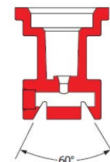
TTJ60-110 VP Spray Tip (Cross Section View)
